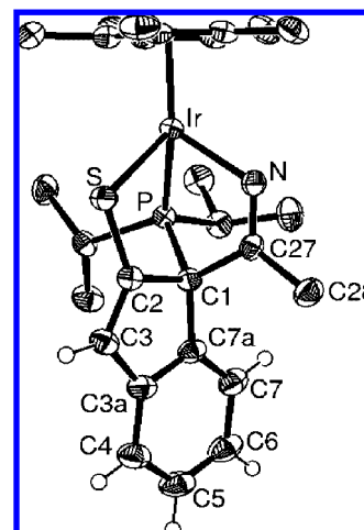
Figure 2. ORTEP diagram for 3·CH 3 CN shown with 50% ellipsoids; selected H-atoms have been omitted for clarity.
