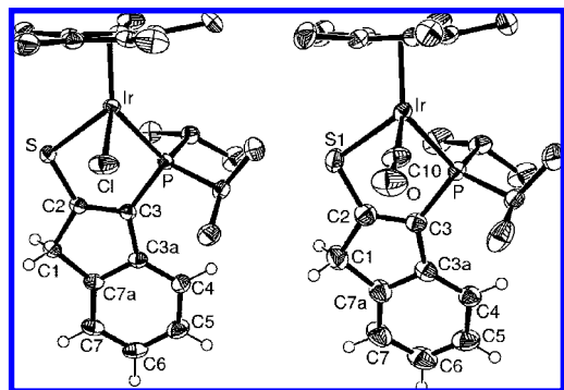
Figure 1. ORTEP diagrams for 1 (left) and [2 \cdot \text{CO}]^+ \text{OTf}^- (right) shown with 50% ellipsoids; selected H-atoms and the triflate counteranion in [2 \cdot \text{CO}]^+ \text{OTf}^- have been omitted for clarity.
